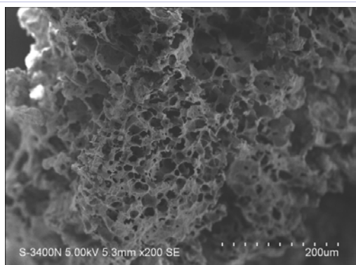
Figure 1c: SEM photographs of interior morphology of the selected gels under investigation for (c) Chitosan/ Brazilian Propolis.
