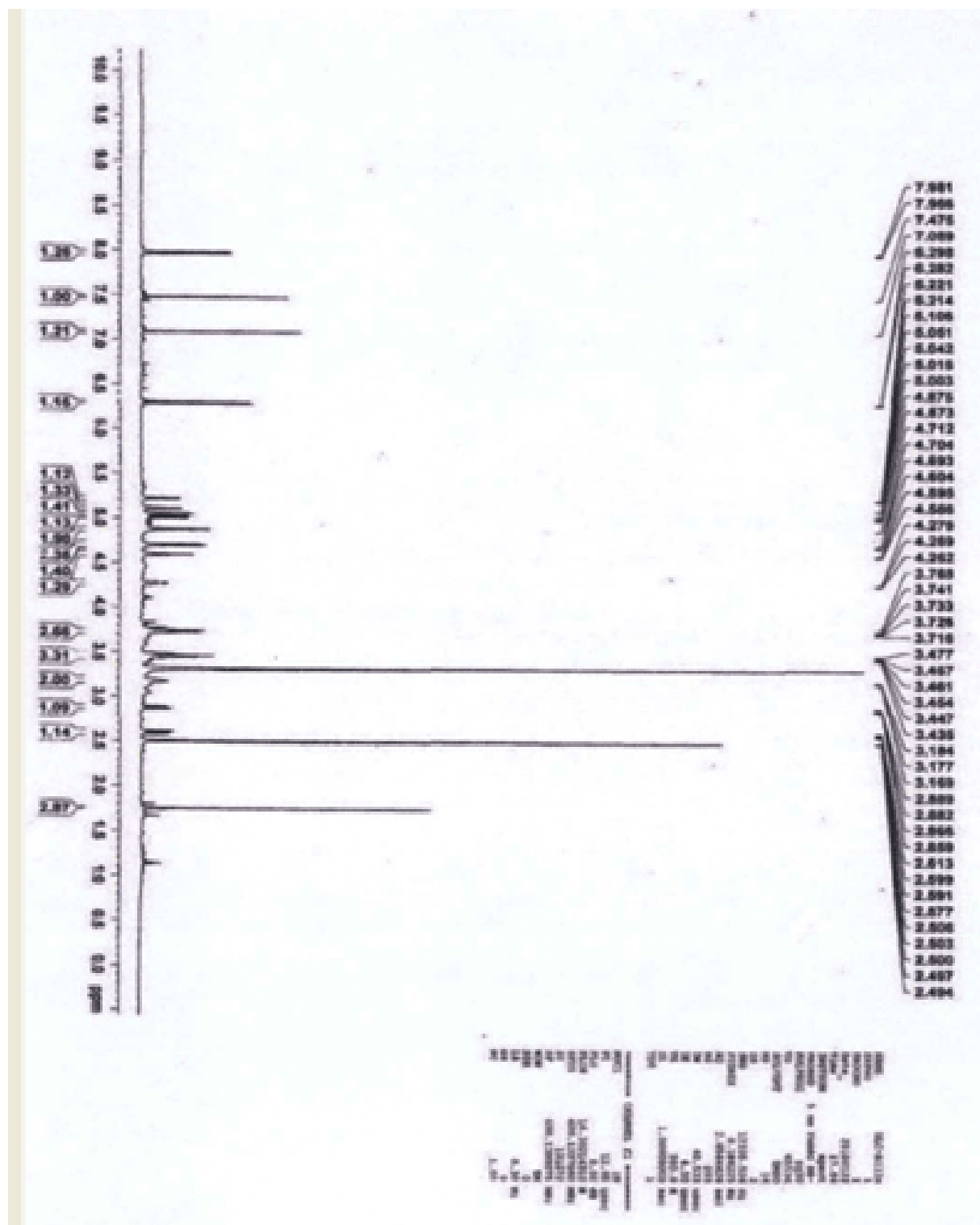
Figure 4: ^1\text{H} NMR spectrum of 1 ( \text{DMSO-}d_6 )
