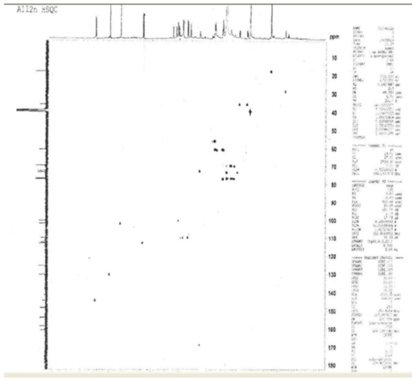
Figure 6: HSQC spectrum of 1 (DMSO- d_6 )
