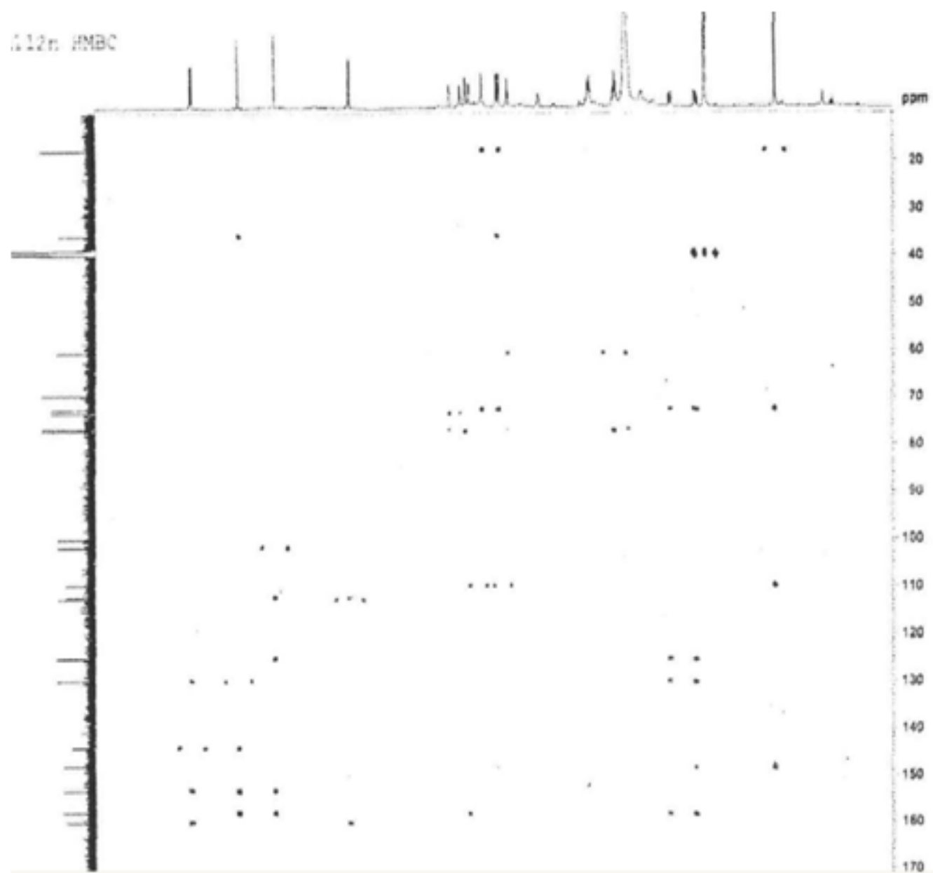
Figure 7: HMBC spectrum of 1(DMSO- d_6 )
