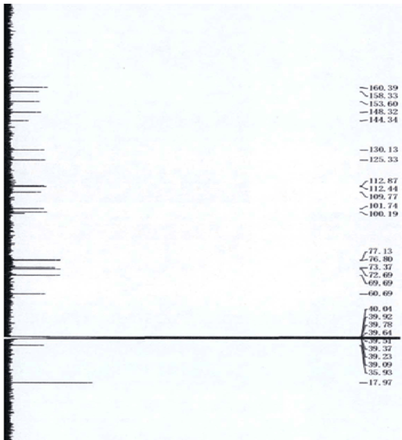
Figure 5: ^{13}\text{C} NMR spectrum of 1 (DMSO- d_6 )
