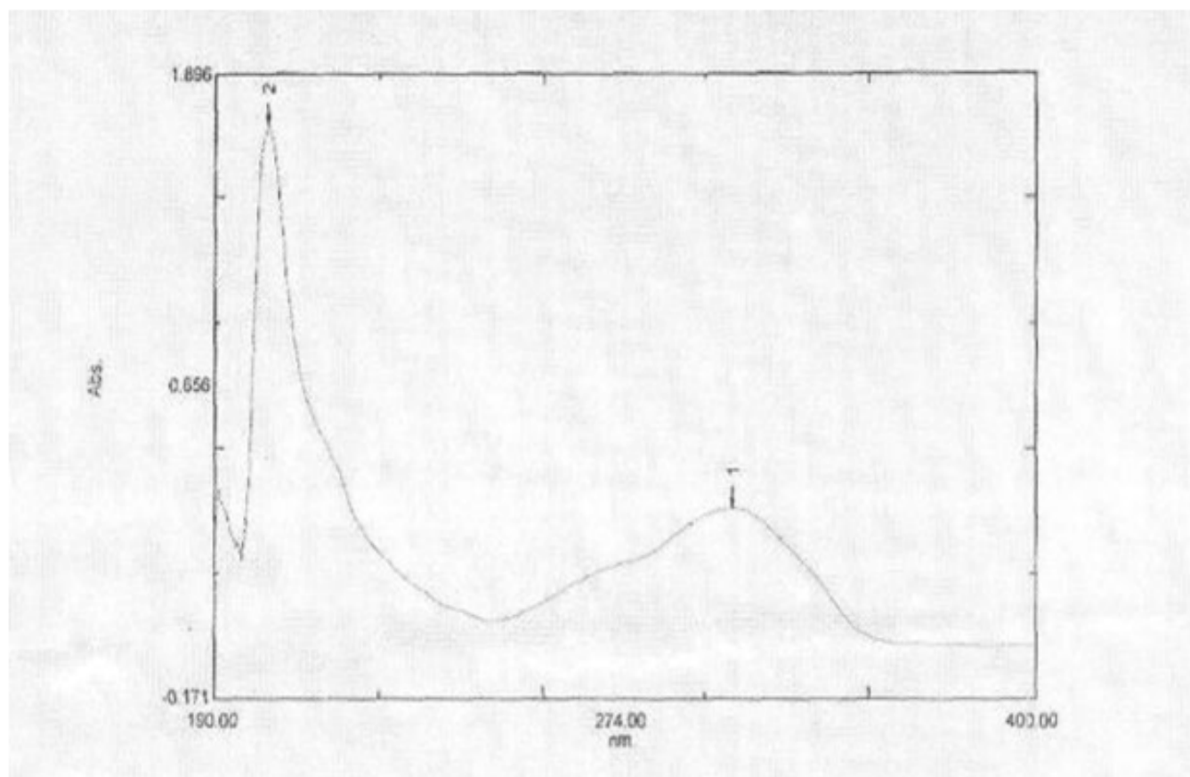
Figure 9: UV spectrum of 2(DMSO- d_6 )
