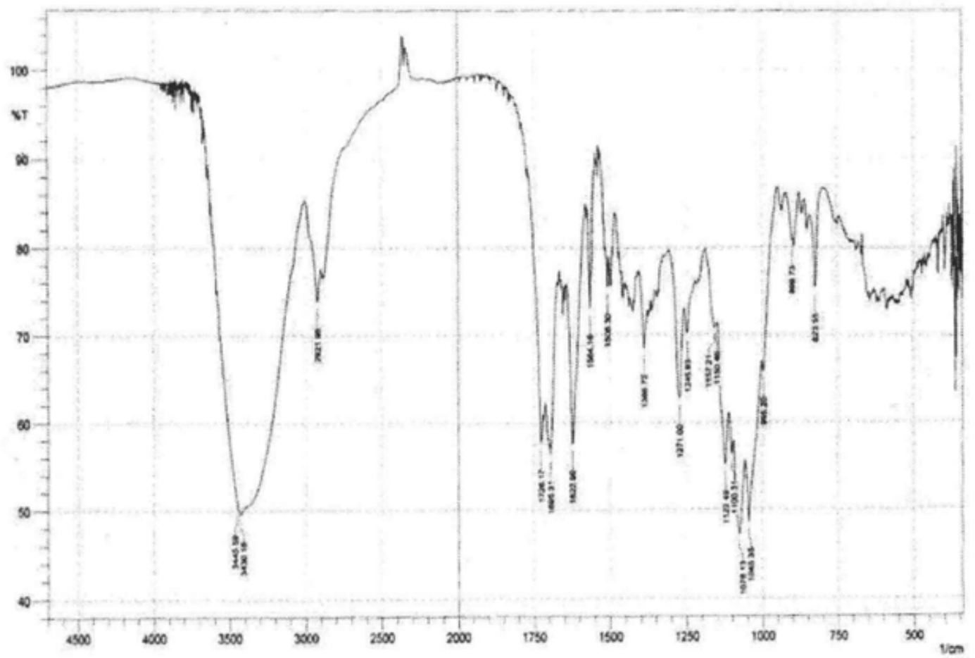
Figure 3: IR spectrum of 1
